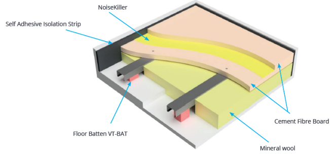
Illustration of a typical installation
